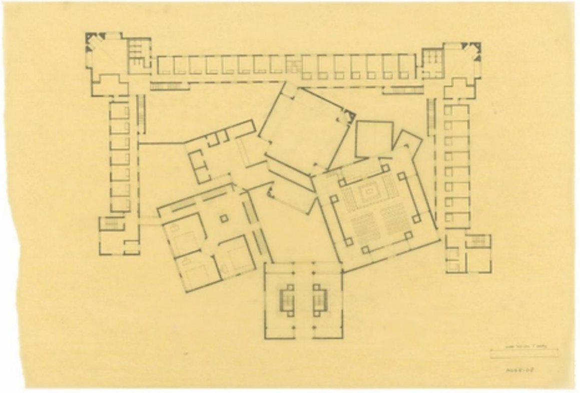
The Dominican Motherhouse, 1965 to 1968.
